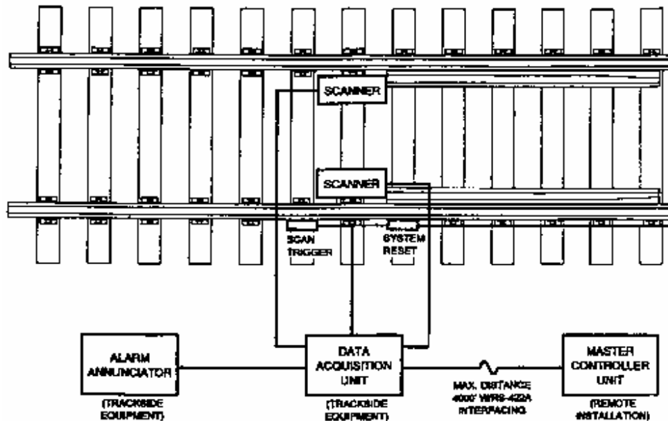
Figure 1: Wheel inspection station - schematic drawing.
