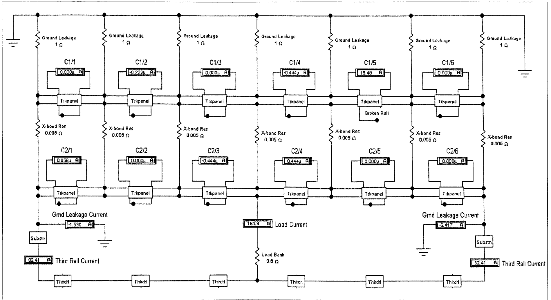
Figure A13. Center shunt method, two interconnected substations, center load bank, one rail break.
