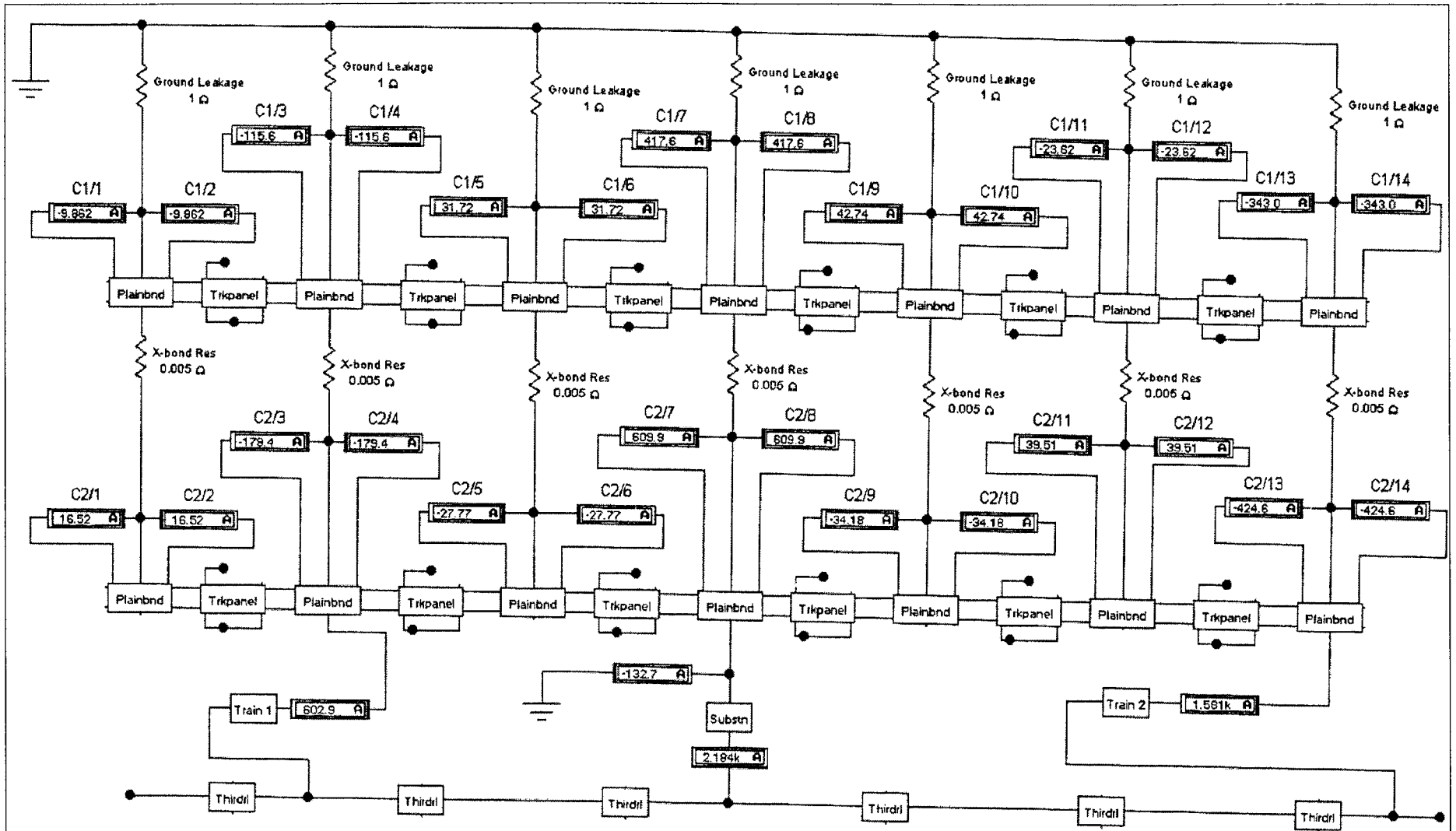
Figure A1. Current difference method, center substation, two trains, no rail break.
