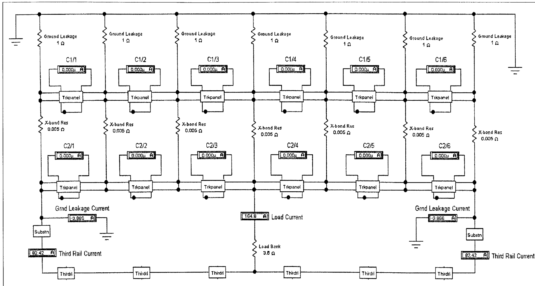
Figure A12. Center shunt method, two interconnected substations, center load bank, no rail break.
