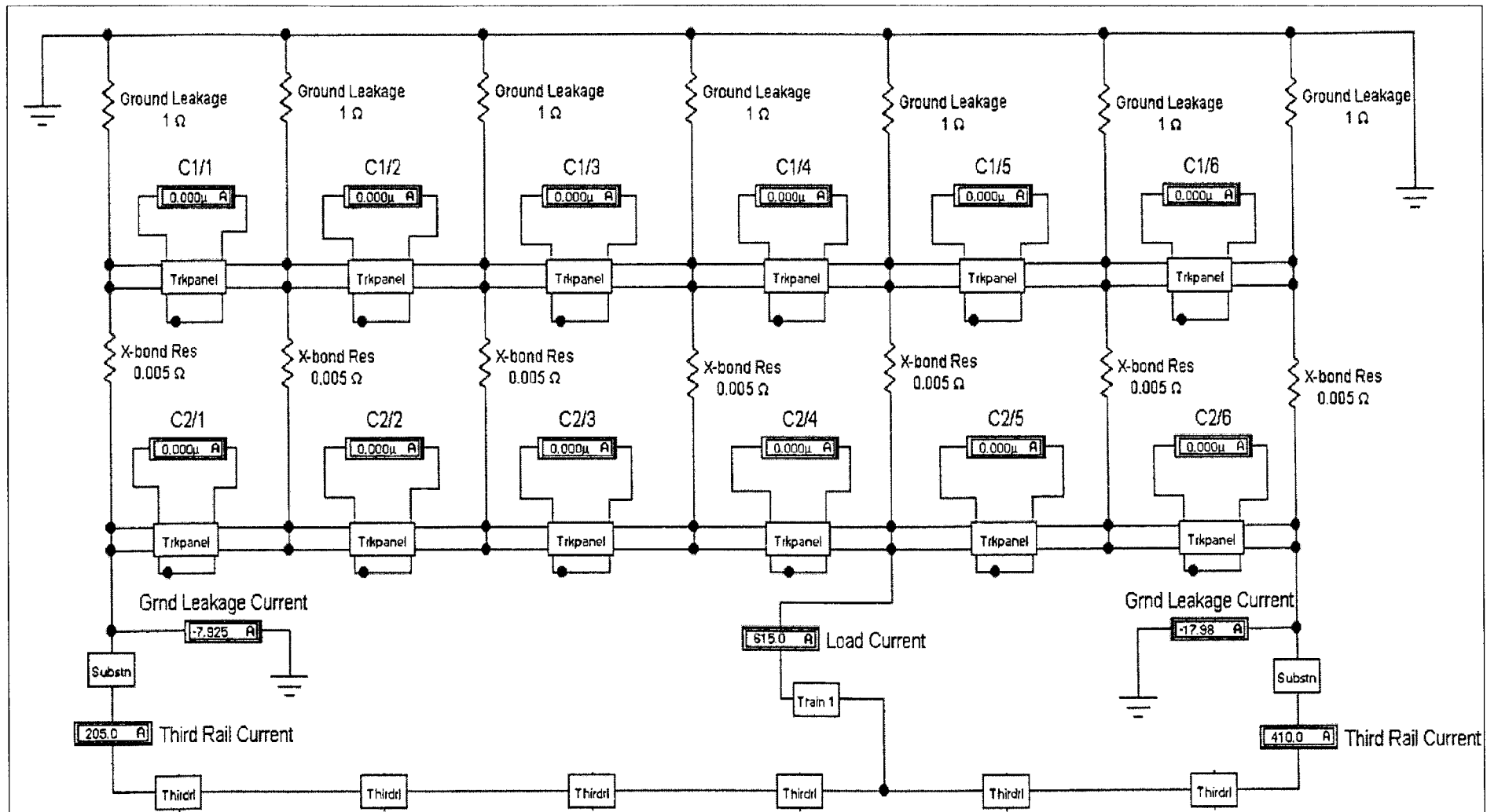
Figure A8. Center shunt method, two interconnected substations, one train, no rail break.
