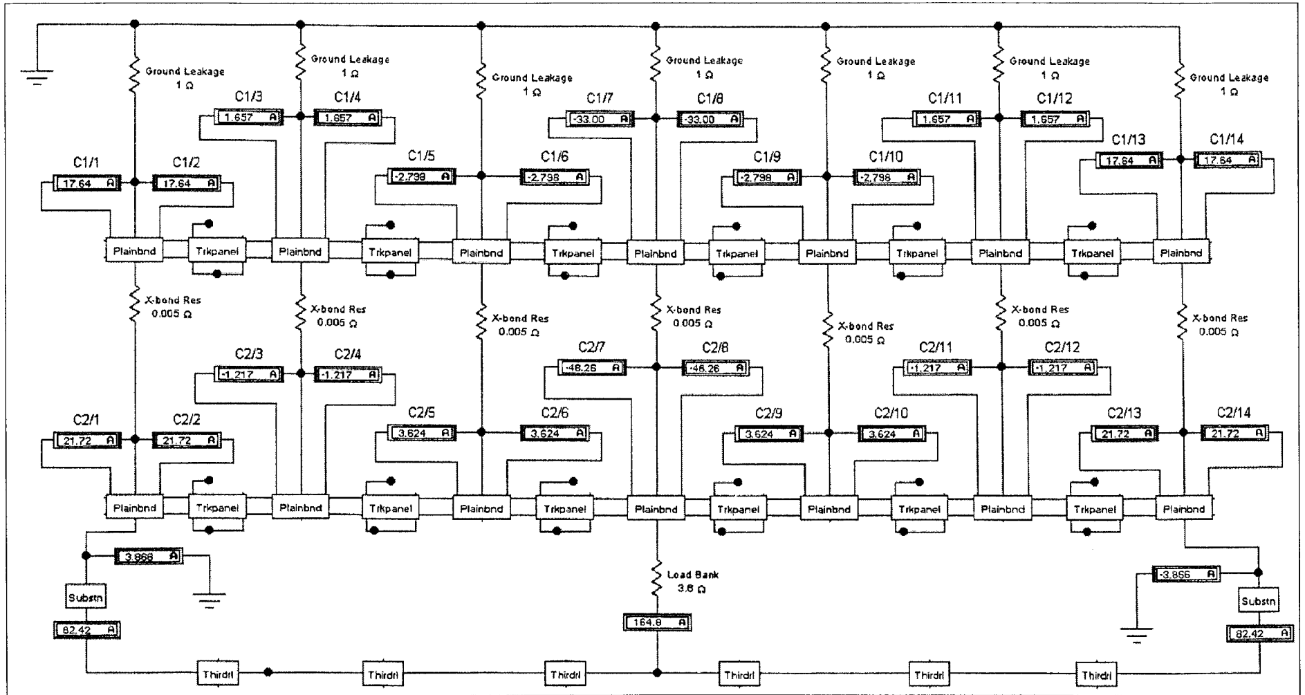
Figure A10. Current difference method, two interconnected substations, center load bank, no rail break.
