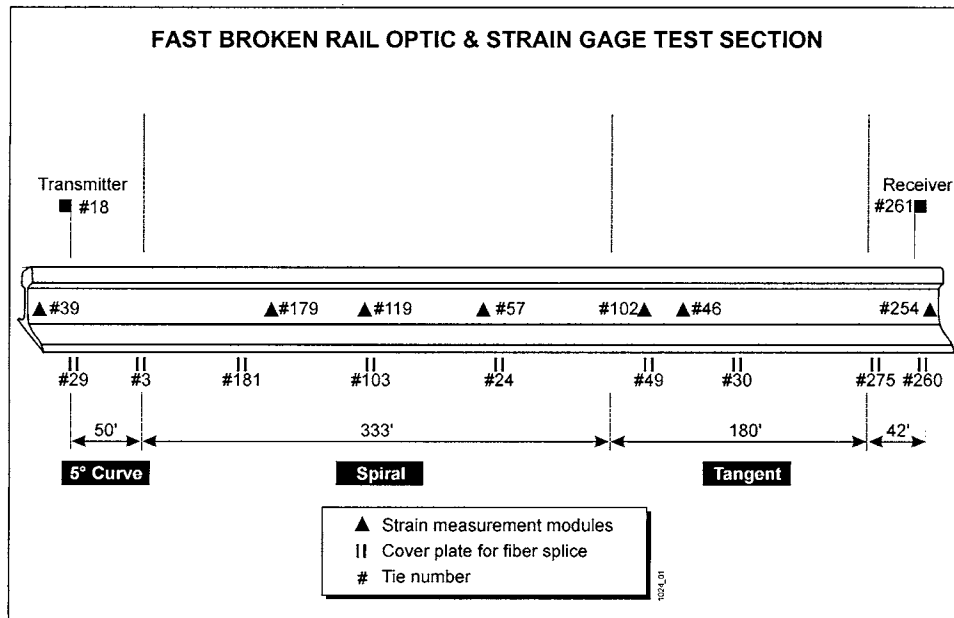
Figure 6. Strain gage and fiber-optic test zone detection system schematic.
