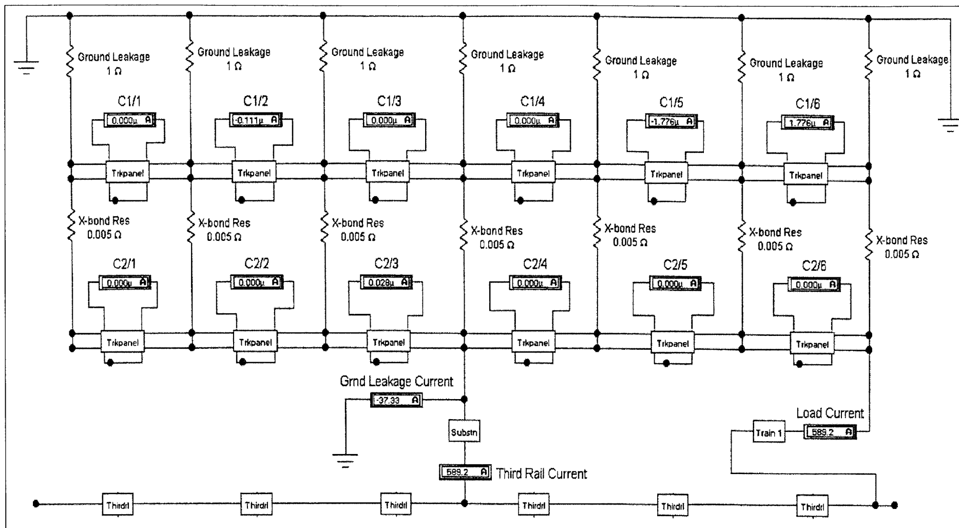
Figure A6. Center shunt method, center substation, one train, no rail break.
