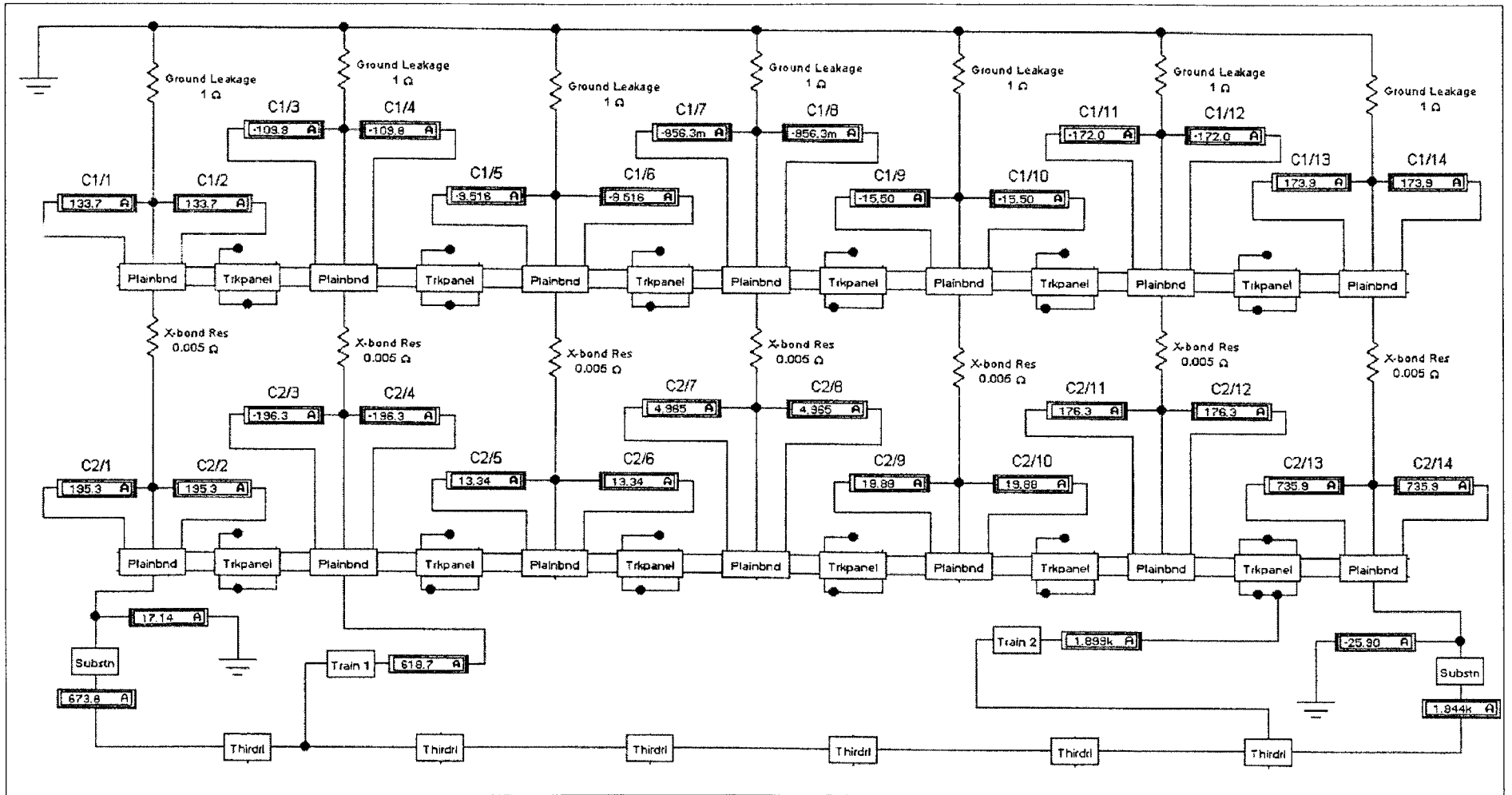
Figure A-3. Current difference method, two interconnected substations, two trains, no rail break.
