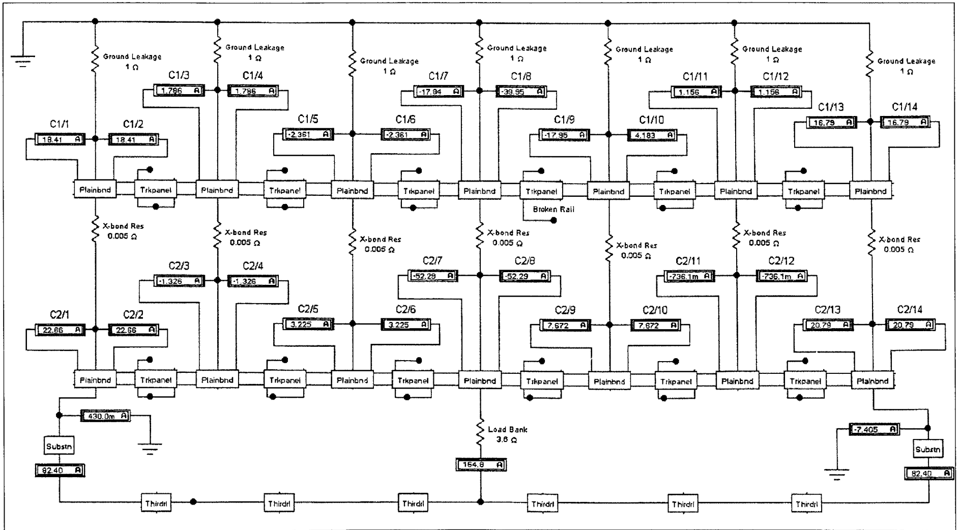
Figure A11. Current difference method, two interconnected substations, center load bank, one rail break.
