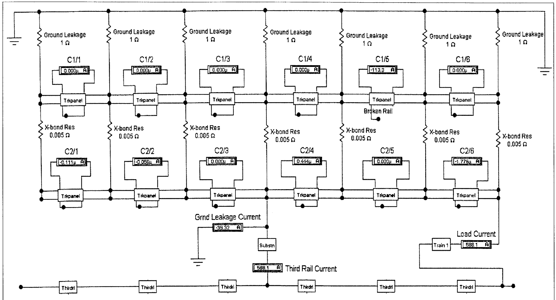
Figure A7. Center shunt method, center substation, one train, one rail break.
