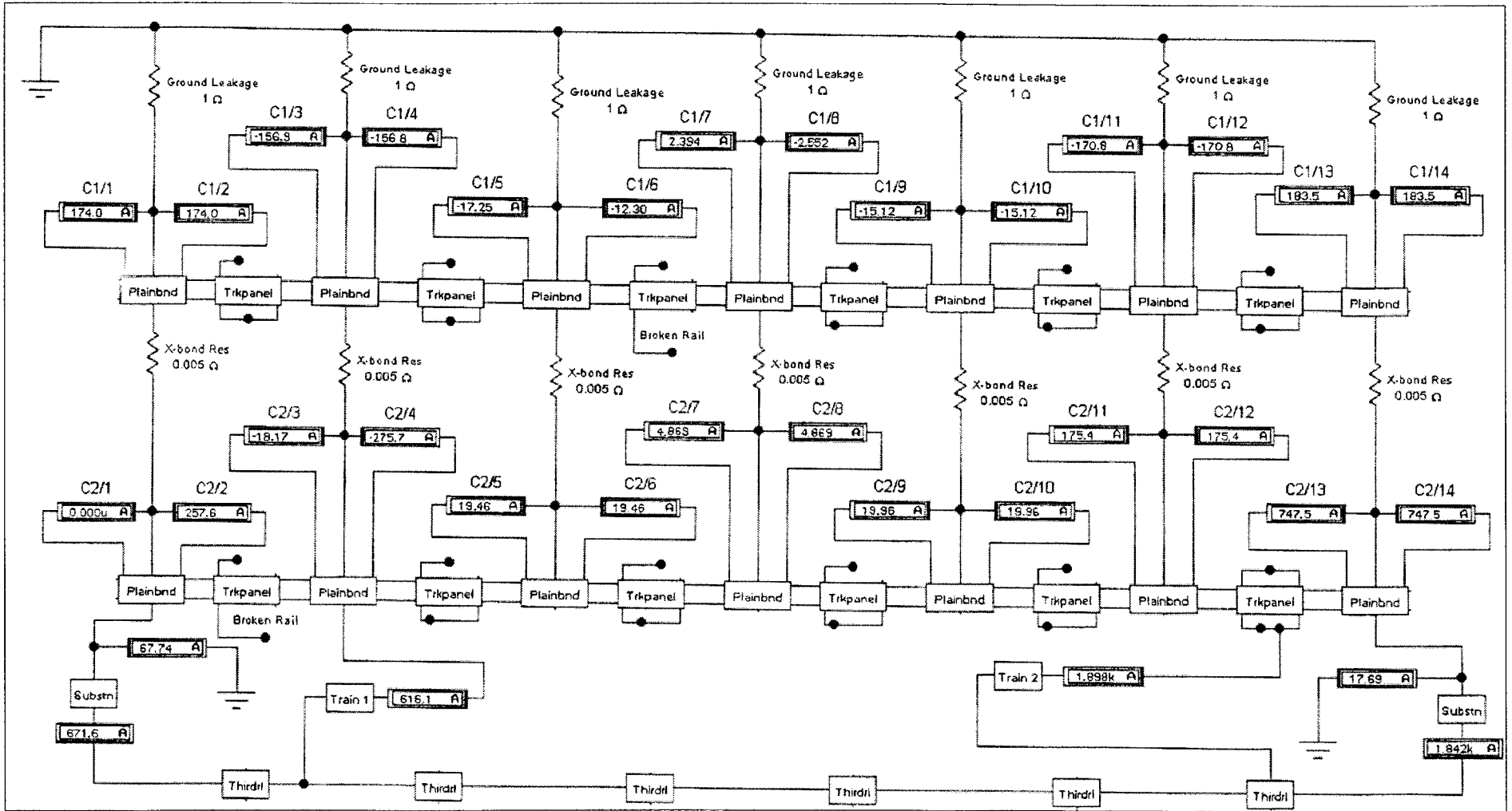
Figure A5. Current difference method, two interconnected substations, two trains, two rail breaks.
