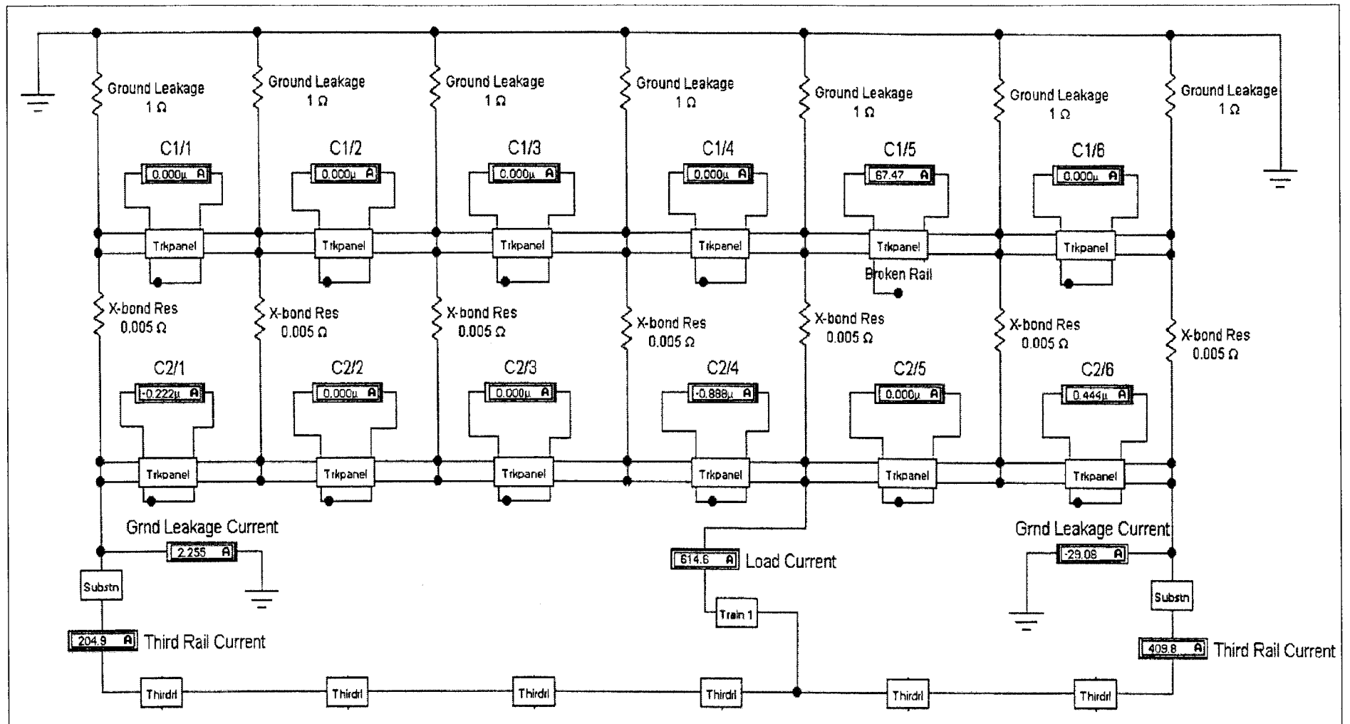
Figure A9. Center shunt method, two interconnected substations, one train, one rail break.
