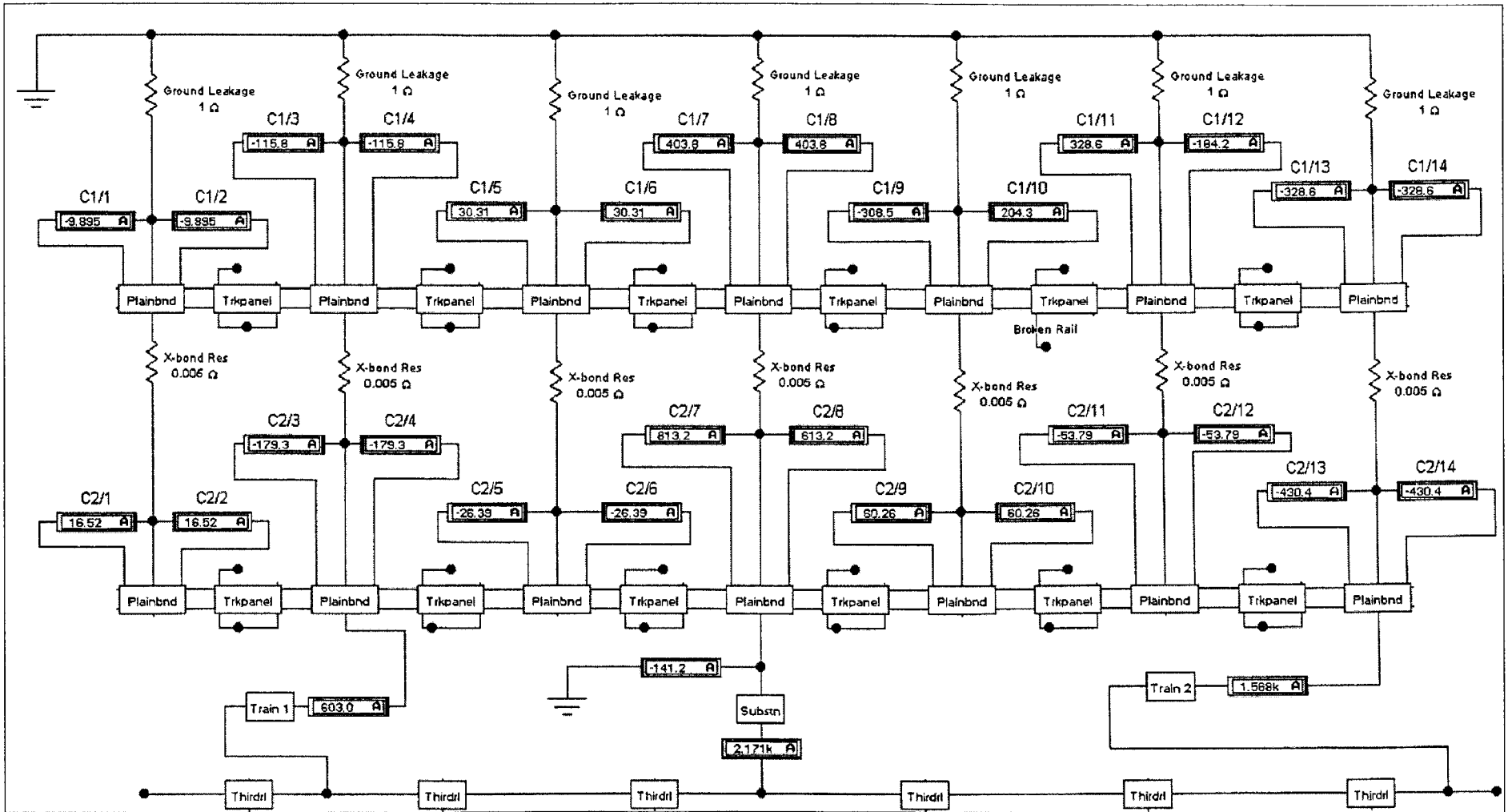
Figure A2. Current difference method, center substation, two trains, one rail break.
