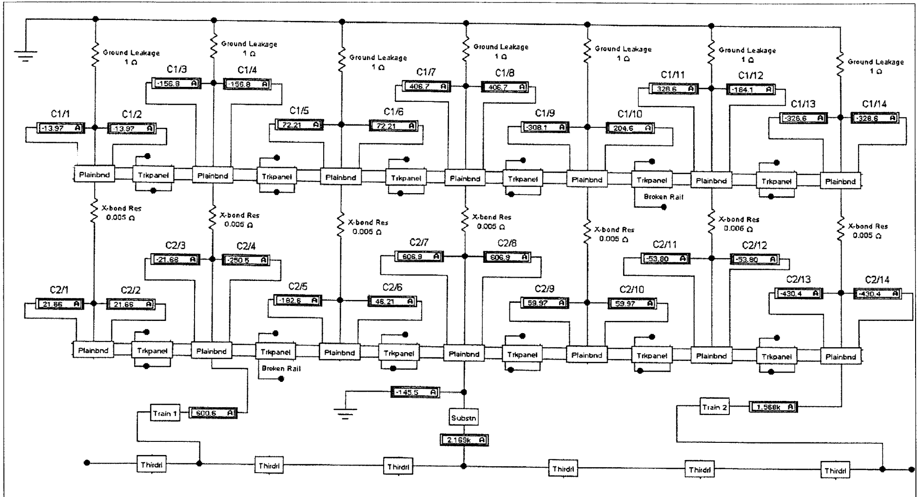
Figure A4. Current difference method, center substation, two trains, two rail breaks.
